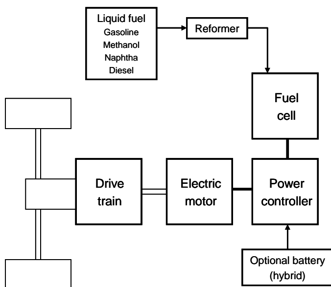
Fig 6.1.3 2010 Indirect FC vehicles
