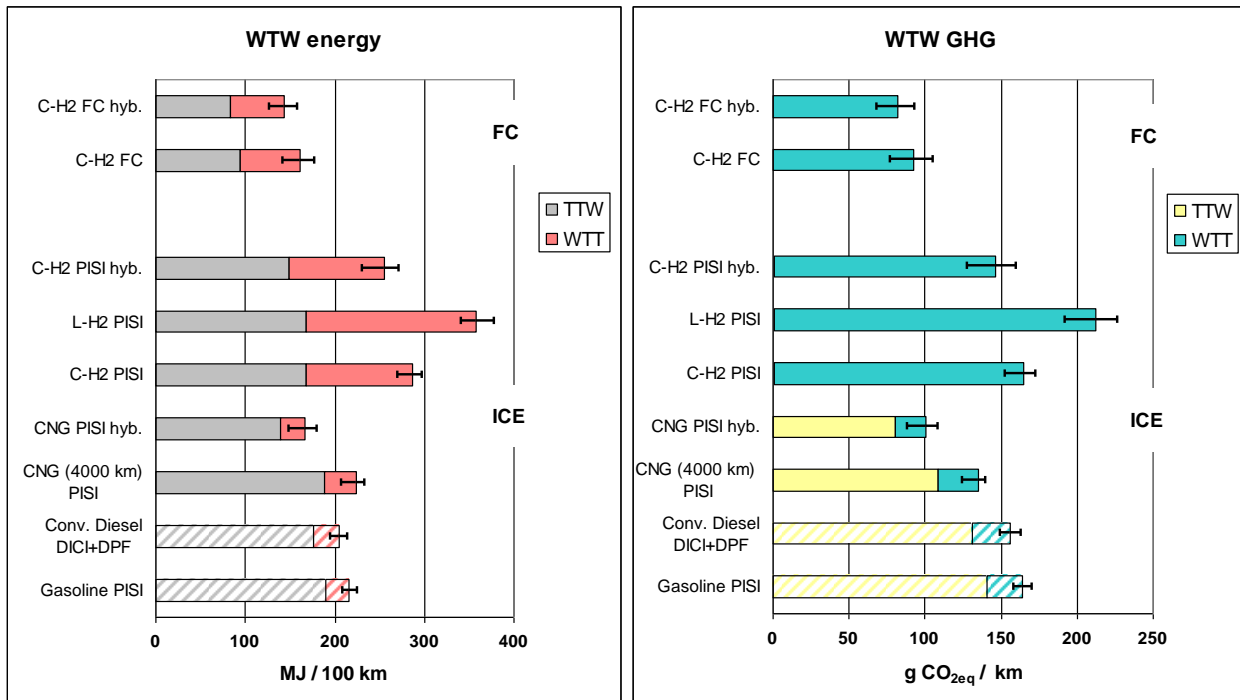
Figure 6.4.1-1a/b WTW total energy requirement and GHG emissions for conventional, CNG and natural gas based hydrogen pathways (2010+ vehicles) (NG source: pipeline 4000 km)
