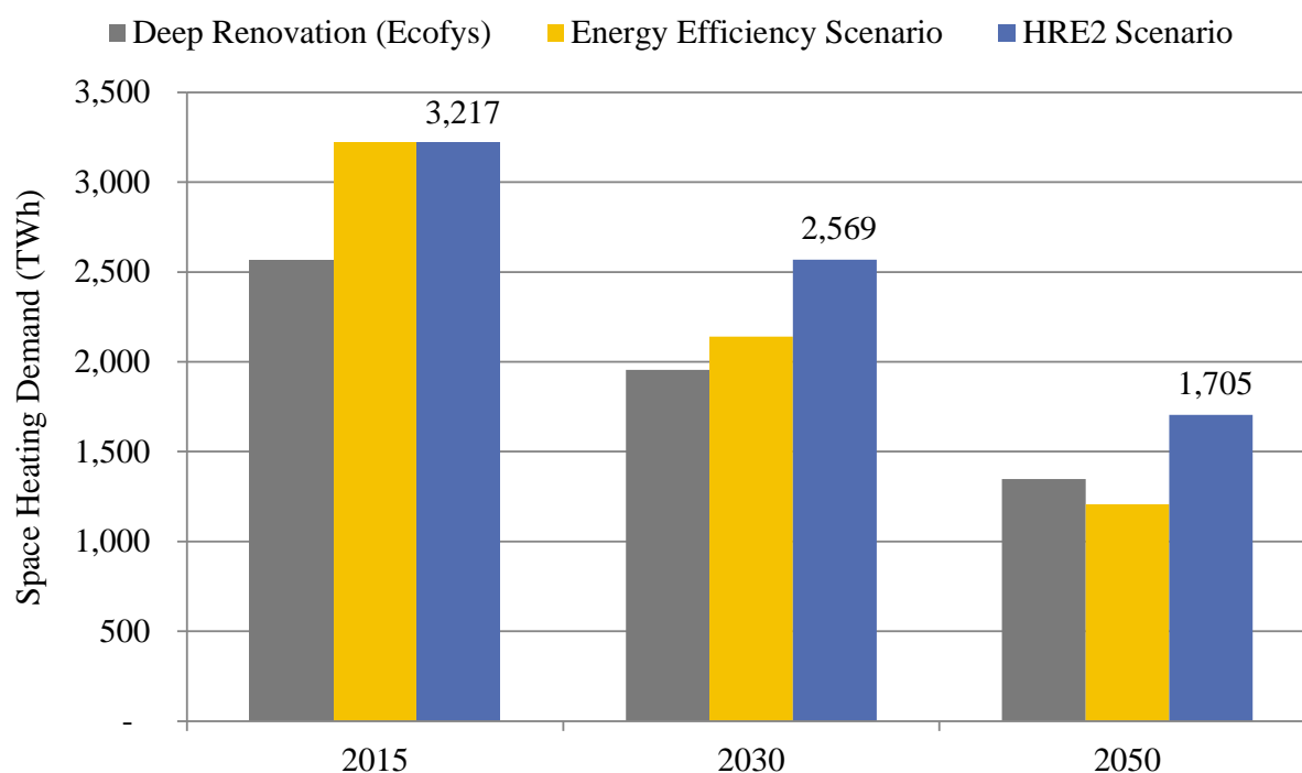
Figure 77: Space heating in the EE scenario from the Energy Roadmap 2050 [9], the Deep Renovation scenario from Ecofys [Boermans, Bettgenhäuser et al., 2012], and the new space heating demand assumed in this study.
