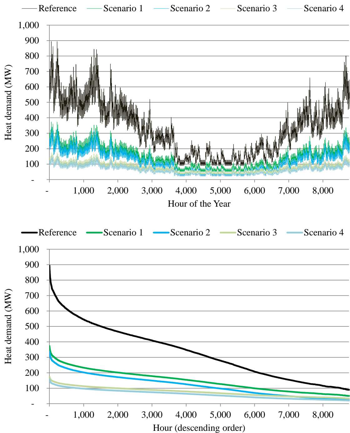
Figure 93: Hourly heat loads for the reference and both scenarios.
