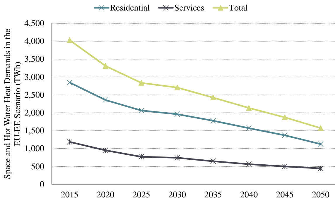
Figure 41: Heat demand for the residential and services sectors separately in the EU-EE scenario between 2015 and 2050.
