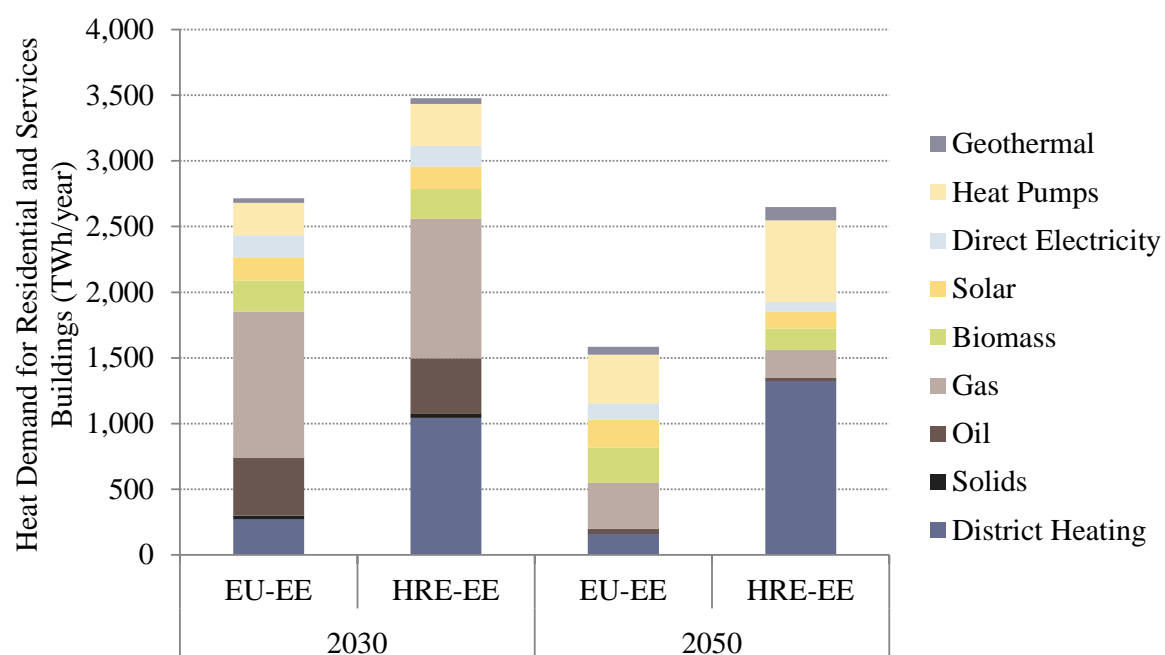
Figure 59: Heat demand by fuel for residential and services buildings in the EU-EE and HRE-EE scenarios for the years 2030 and 2050.
