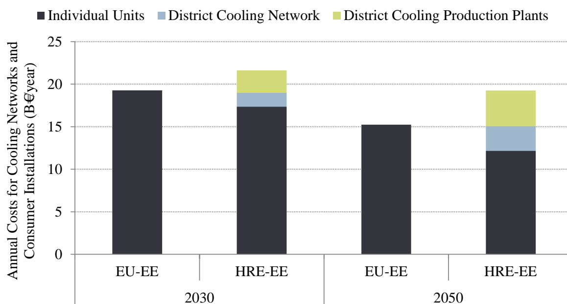
Figure 55: Annual cooling system costs for the EU-EE and HRE-EE scenarios for the years 2030 and 2050.
