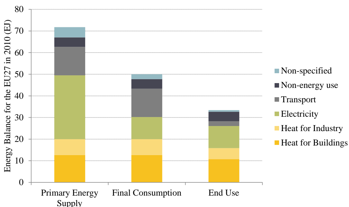
Figure 7: The energy balance in three steps during 2010 for EU27. The energy flows labelled as heat for industry and building include only fuels and district heating. Electricity used for heating is included in the electric energy flows [3].
