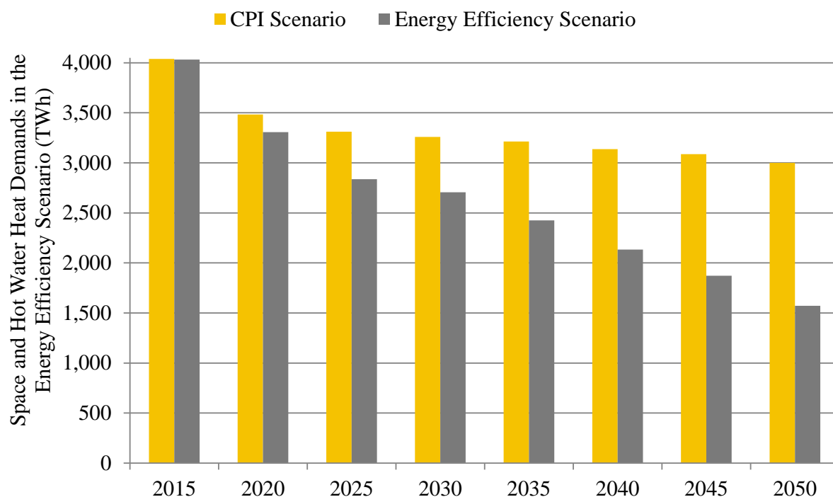
Figure 68: Total heat demand in the EU-CPI and EU-EE scenarios for 2015-2050.
