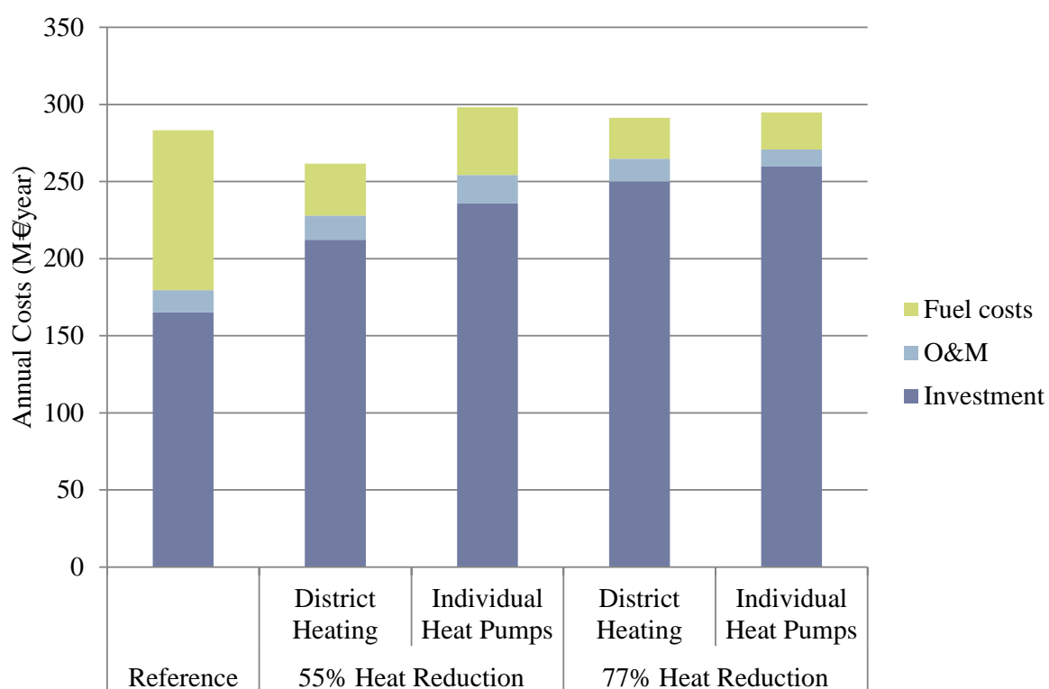
Figure 5: Annualised costs for all scenarios considered in the Aarhus case study.
