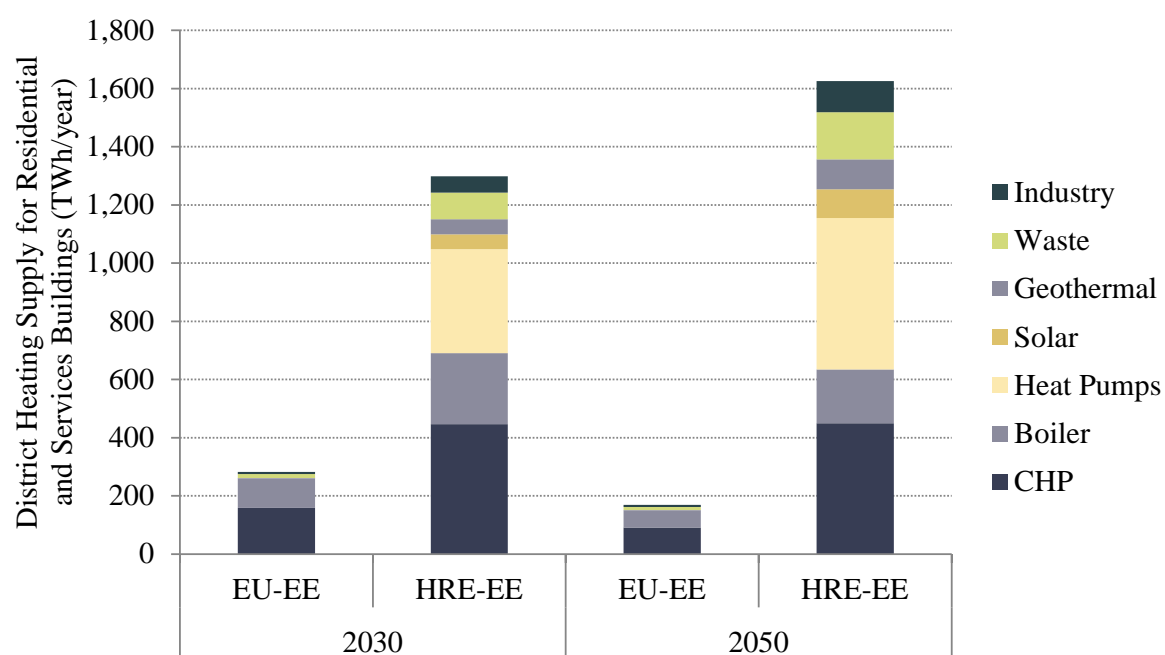
Figure 60: District heating production by plant type in the EU-EE and HRE-EE scenarios for the years 2030 and 2050. Note: some of the district heating is used by absorption heat pumps to provide cooling as discussed in section 5.2.
