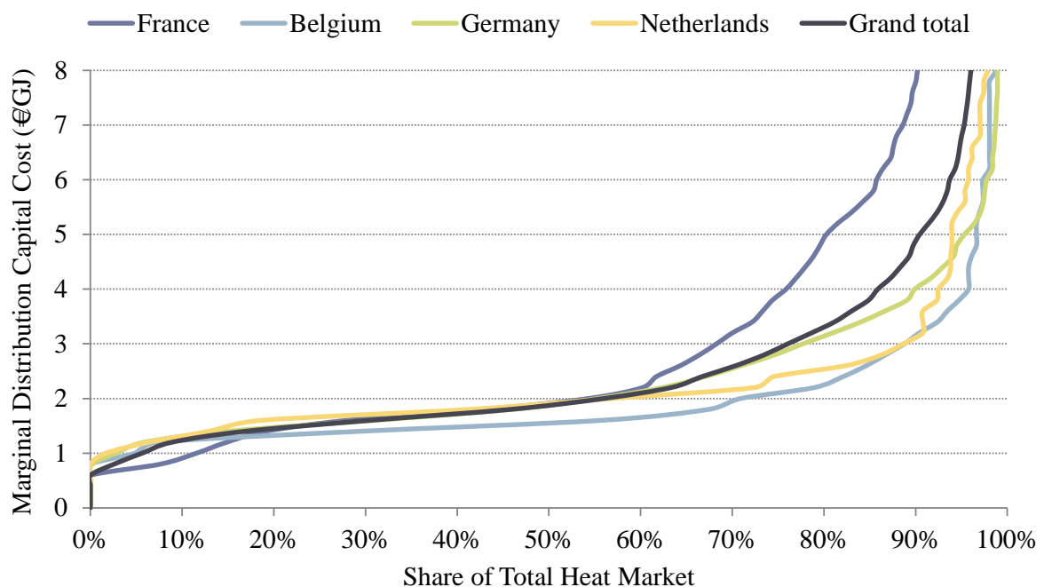
Figure 23: Current marginal distribution capital cost levels and corresponding urban district heating heat market shares in four studied European countries in 2008 [41].
