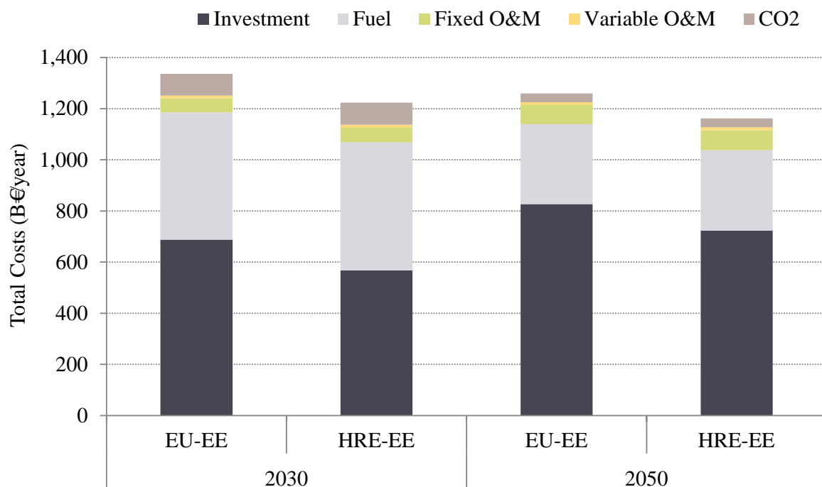
Figure 63: Total annual energy system costs for the EU-EE and HRE-EE scenarios in the years 2030 and 2050.
